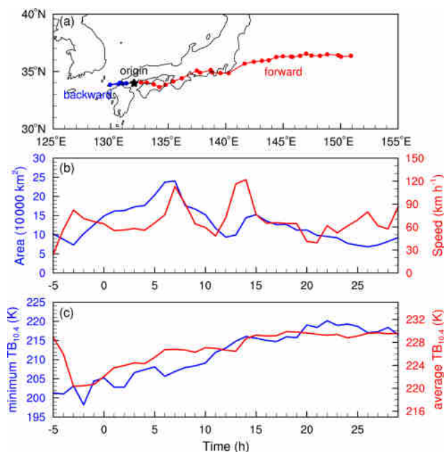
Figure 9. (a) Moving track of the MCS occurring at 13:00 UTC on 20 June 2016 and (b) temporal variations in the area, speed, and (c) minimum and average 10.4\text{ }\mu\text{m} brightness temperature of the MCS.
