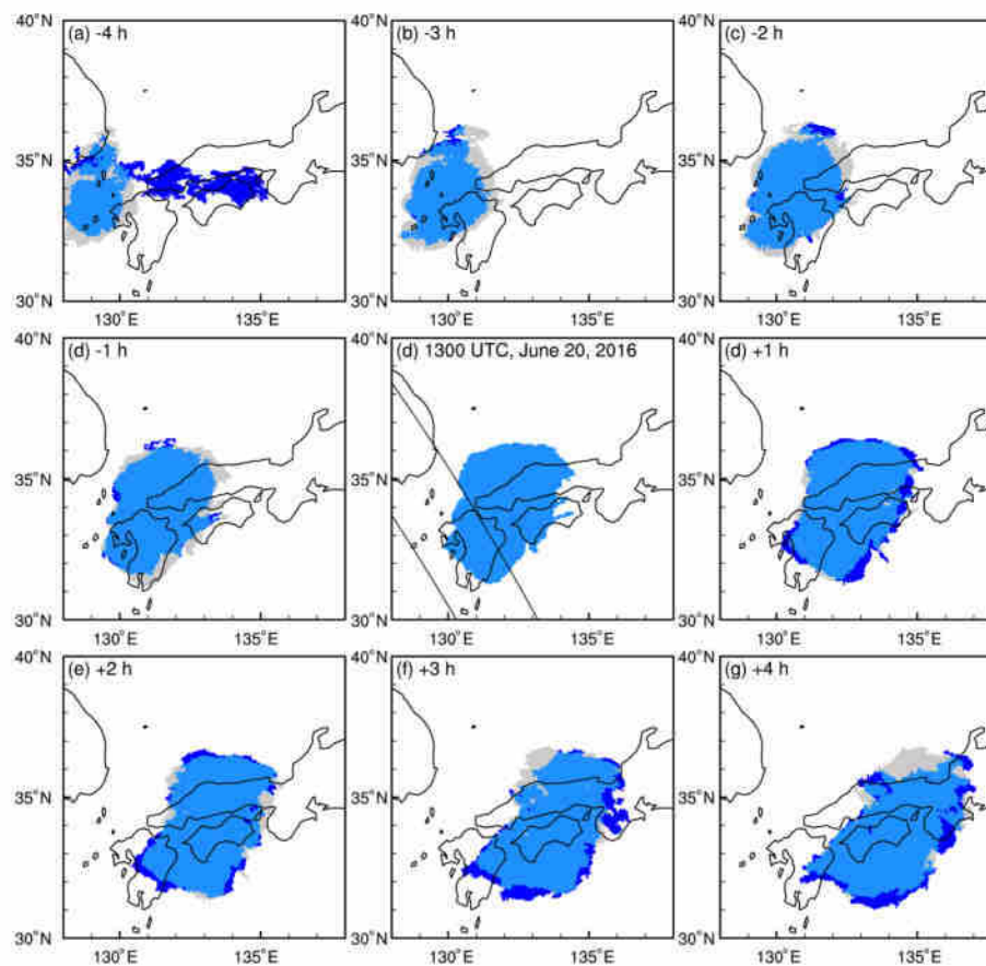
Figure 8. Demonstration of the tracking process for the precipitation event occurring at about 13:00 UTC on 20 June 2016. The light blue and deep blue areas indicate the actual MCS. The gray and light blue areas indicate the calculated MCS from the last record.
